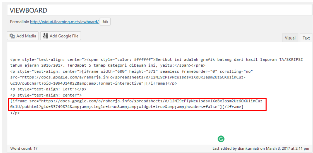
Gambar 10. Script embed
